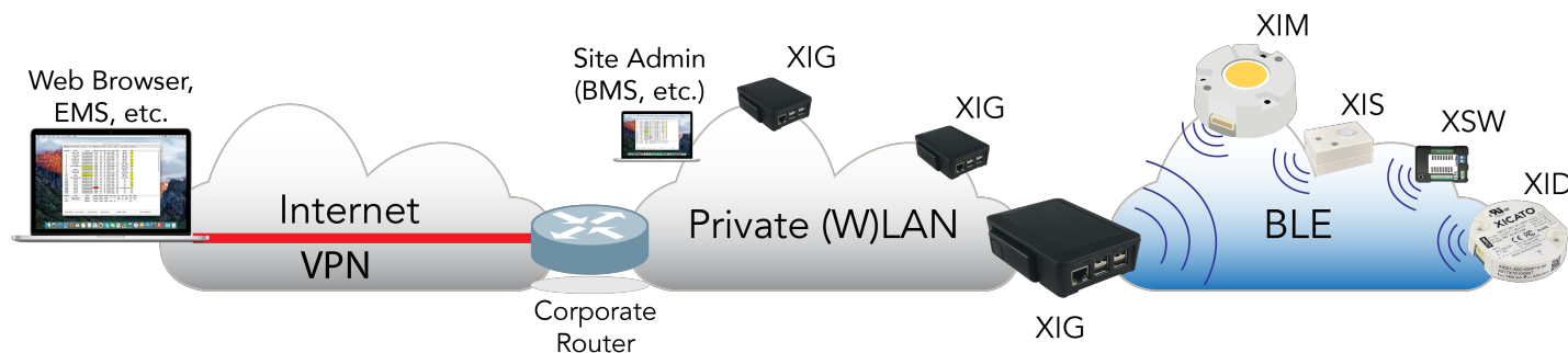
Figure 3: XIG access can be over LAN or Internet VPN using a web browser, EMS/BMS, or 3 rd party control software
